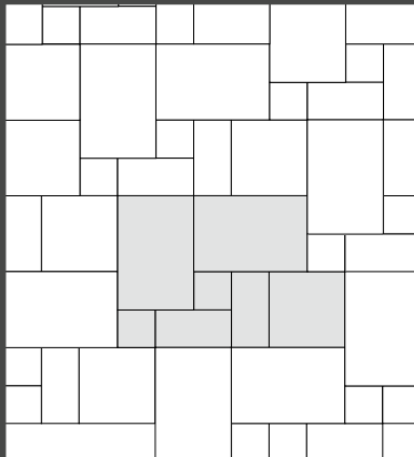
40,6x60,9=55% 40,6x40,6=18% 20,3x40,6=18% 20,3x20,3=9% L
