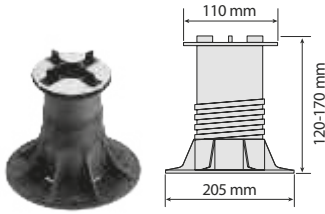
201005 V160 Supporto regolabile autolivellante Adjustable paving support self leveling head mm 120/170
