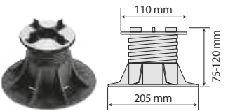
201004 V150 Supporto regolabile autolivellante Adjustable paving support self leveling head mm 75/120
